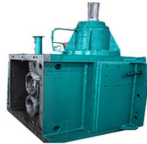
Transmission Gearbox
